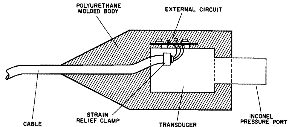
GULTON WAVE SENSOR ASSEMBLY
